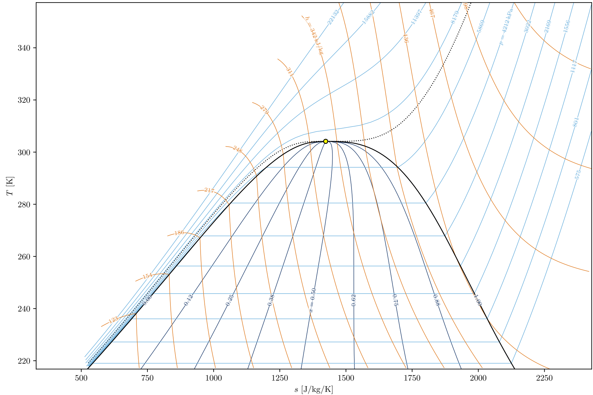
Thermodynamic Diagram (TS) – CO2
